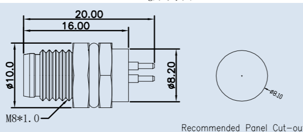
Scale drawing/尺寸图
