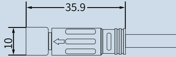
Scale drawing/尺寸图
