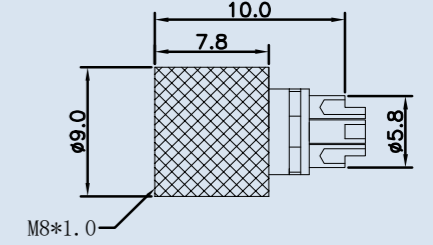
Scale drawing/尺寸图
