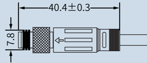
Scale drawing/尺寸图
