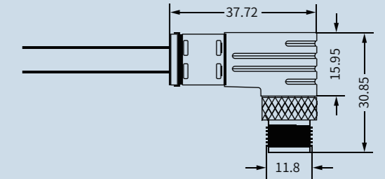
Scale drawing/尺寸图
