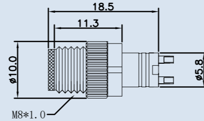
Scale drawing/尺寸图
