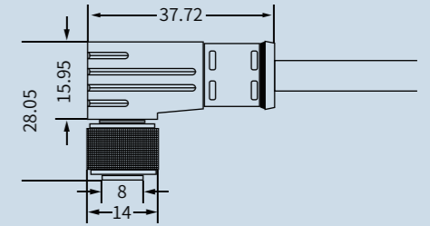
Scale drawing/尺寸图
