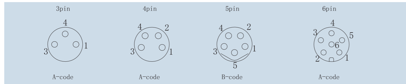
Pin assignment front view/针位分布前视图
