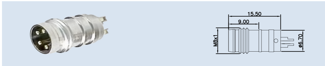
Pin assignment front view/针位分布前视图
