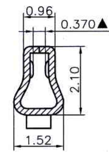
SEC: C-C
