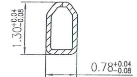
SEC:C-C
