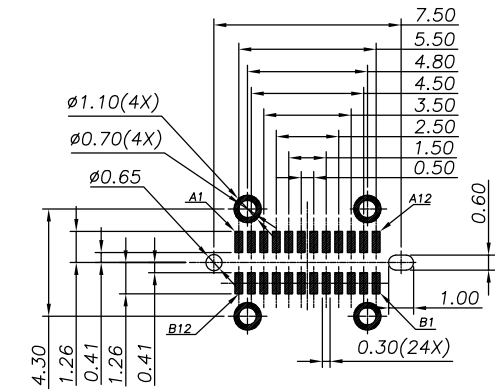
RECOMMENDED PCB LAYOUT(TOP VIEW) THICKNESS 1.0±0.10MM;DEFAULT TOLERANCE:±0.05
