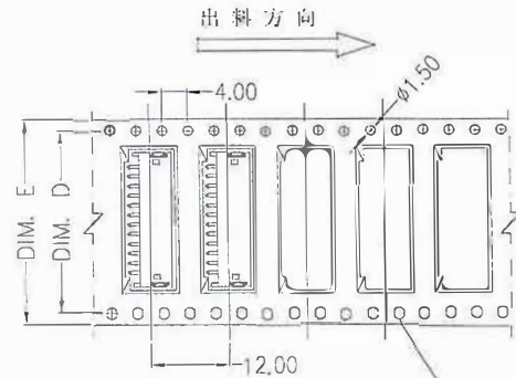
10~14 CONTACTS
